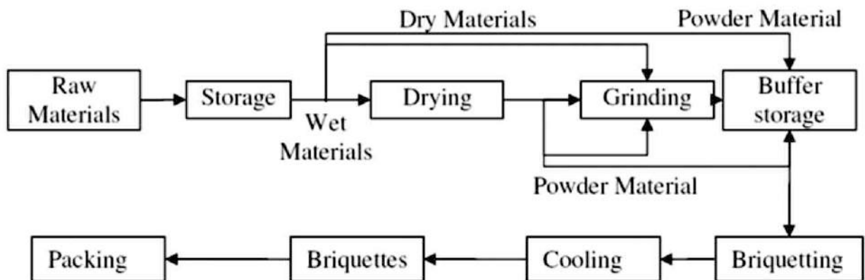
Flow Diagram of Biomass Briquette Production
