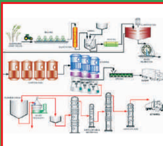
Bio-ethanol Extraction Process through Sugarcane
